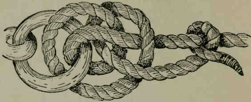
FIG. 53.—Fisherman's hitch.
